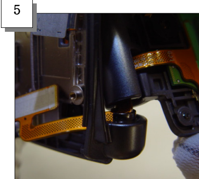
Put LCD FPCB in the Front Hinge
