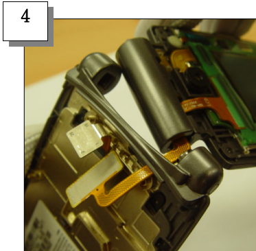
Put LCD FPCB in the Front Hinge
