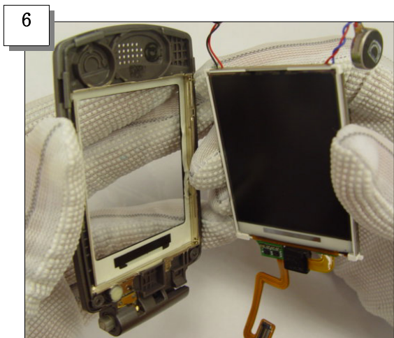
Disjoint the LCD from the Lower
