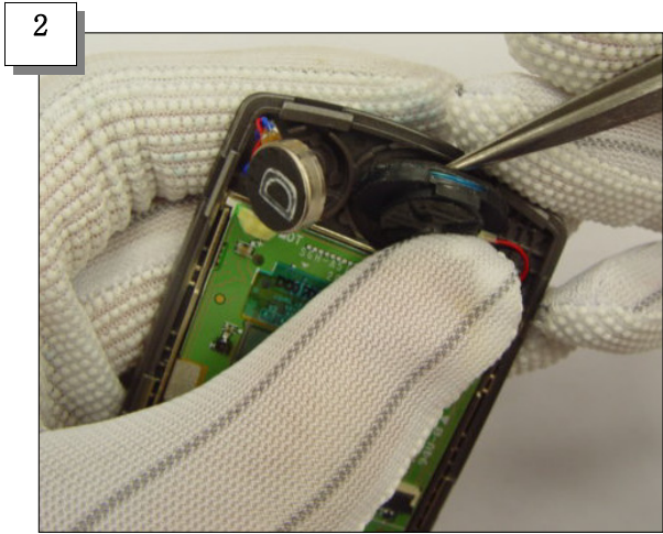
Draw the Speaker out
