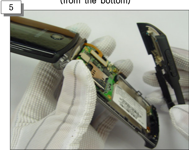
Open the side with a knife (from the bottom)
