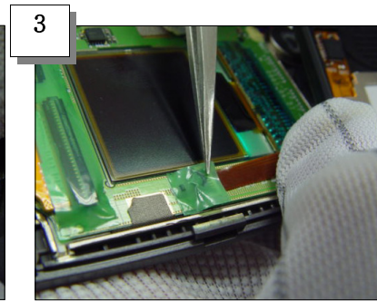
3 Attach the Tape on the Connector
