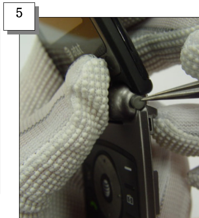
5 Remove the Rubber beside the Front
