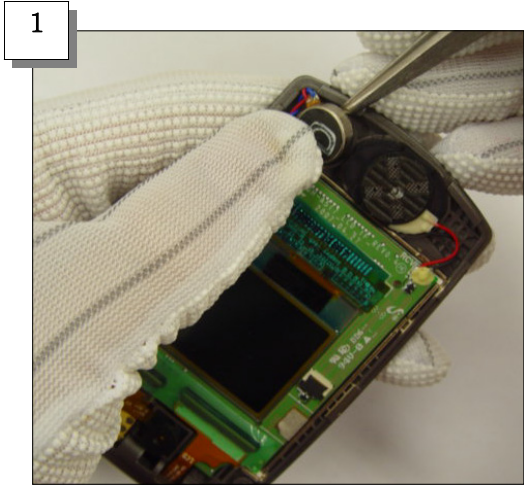
Draw the Motor out
