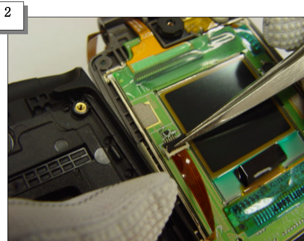
Open the Connector
