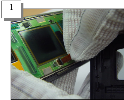
1 Join the Touch key to the connector
