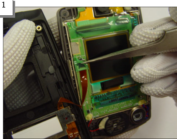
Remove the Tape on the Connector
