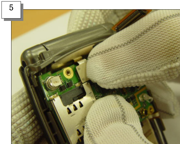
Assemble the Key Connector
