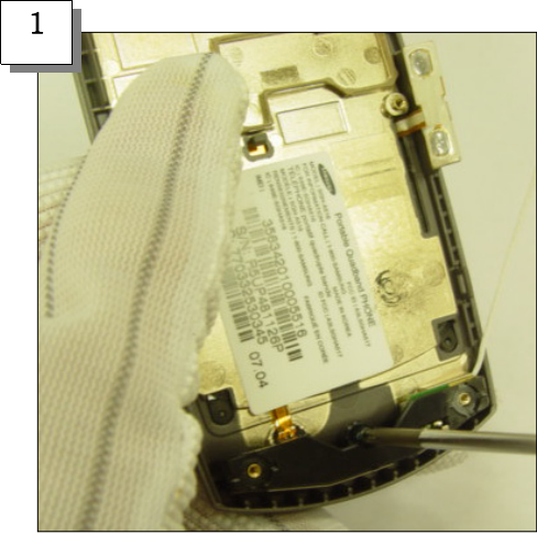
Join the Screw to the Antenna
