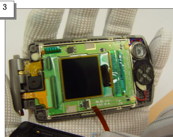
Draw the FPCB out
