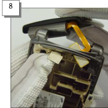
8 Draw out the LCD Connector from Front
