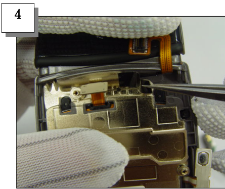
4 Remove the Dustproof Tape
