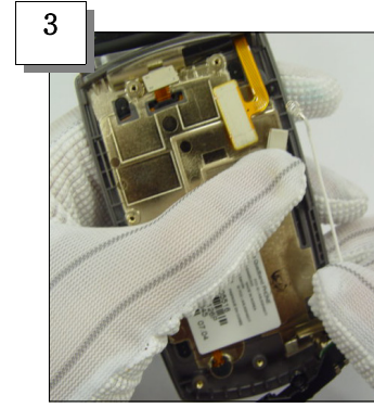
3 Disjoint the Antenna & Wire
