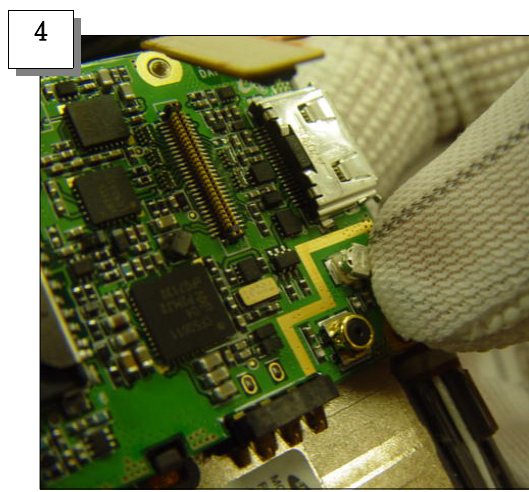
Join the Antenna switch to the PBA
