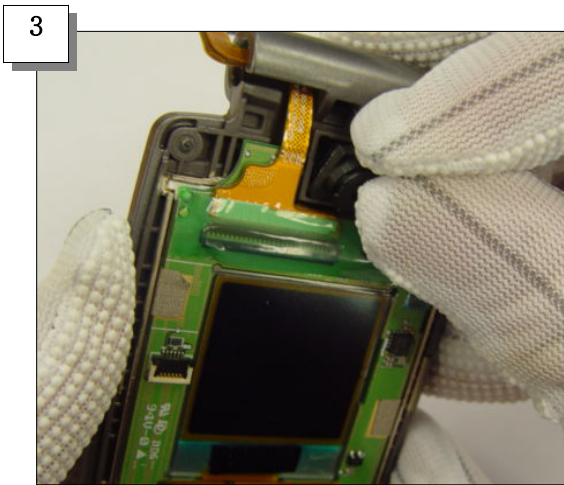
Draw the Camera out
