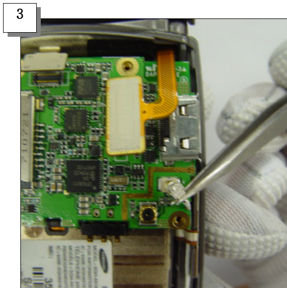
Disjoint the Antenna Switch
