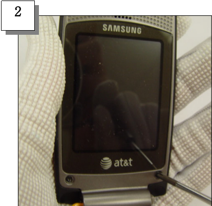
2 Remove the Screws (2 Points)
