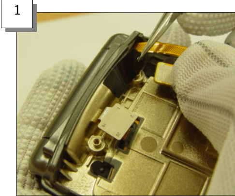
Attach the Dustproof Tape
