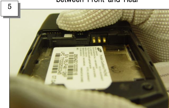
Join the Center part so that hooker is locked correctly
