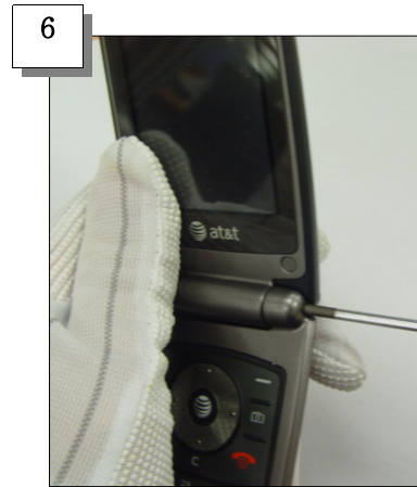
6 Press the Hinge with a lever
